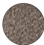
Shale
